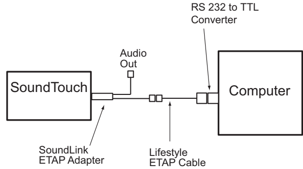
ETAP Block Diagram
