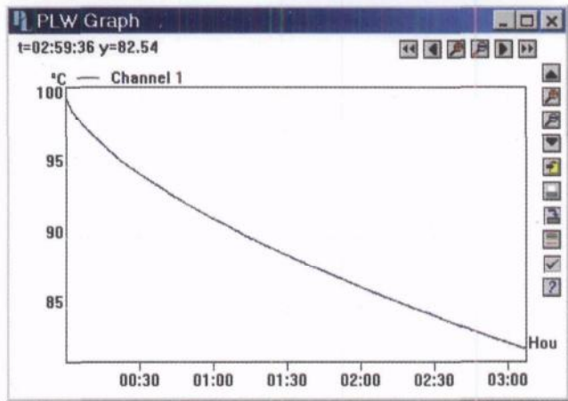
Figure 1 - RHC made with wood basket
