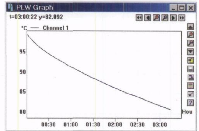
Figure 2 - RHC made with a cardboard box
