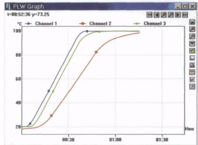
Figure 6 - Internal temperature lag of food in RHC
