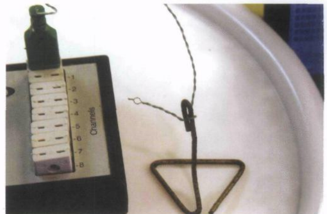
Photo 1 - Thermocouple Support
