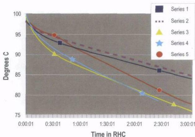
Figure 5 - Comparison of various RHC properties
